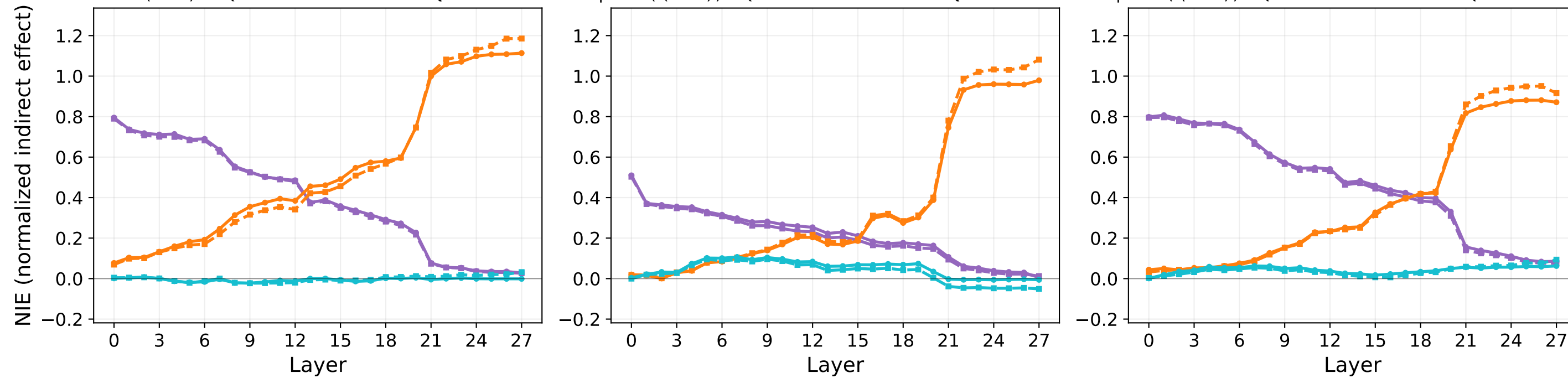
Qwen2.5-1.5B within-model (solid) vs Qwen2.5-1.5B-Instruct → Qwen2.5-1.5B within-model (solid) vs Qwen2.5-1.5B-Instruct → Qwen2.5-1.5B cross-patch (dashed) (j) Gender — Words NIE (k) Race — Words NIE (l) Profession — Words NIE
