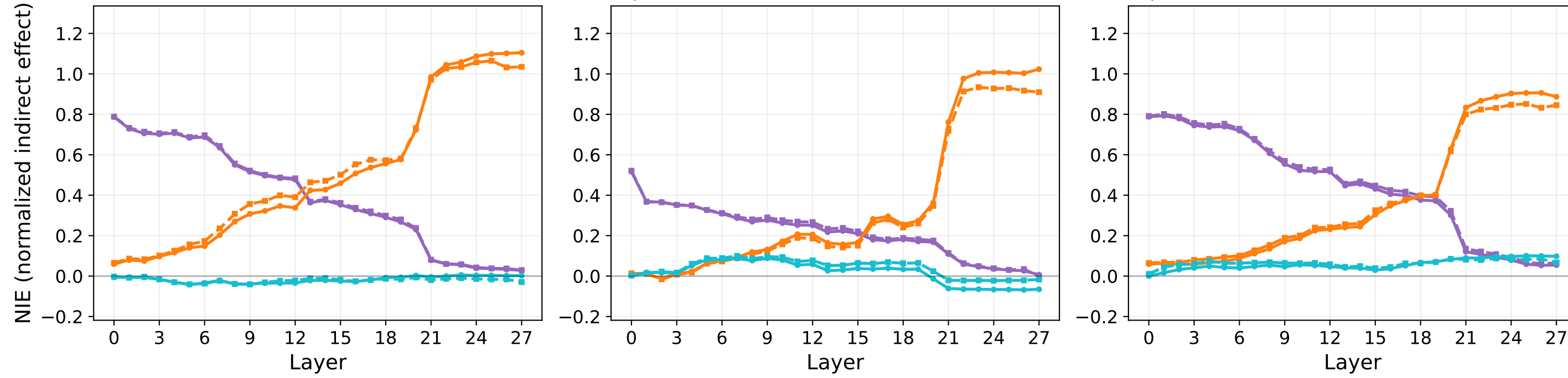
Qwen2.5-1.5B within-model (solid) vs Qwen2.5-1.5B-Instruct → Qwen2.5-1.5B within-model (solid) vs Qwen2.5-1.5B-Instruct → Qwen2.5-1.5B cross-patch (dashed) (g) Gender — States NIE (h) Race — States NIE (i) Profession — States NIE
