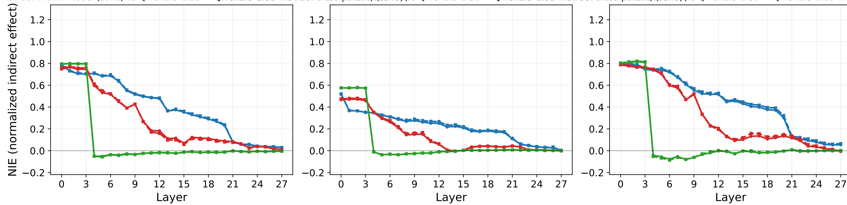
Qwen2.5-1.5B-Instruct within-model (solid) vs Qwen2.5-1.5B → Qwen2.5-1.5B-Instruct cross-patch (dashed) (d) Gender — Words NIE (e) Race — Words NIE (f) Profession — Words NIE
