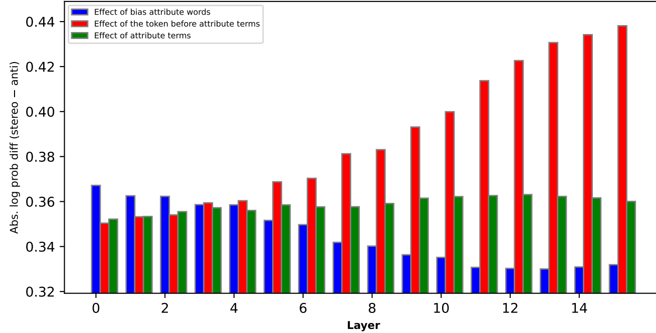
step2600
