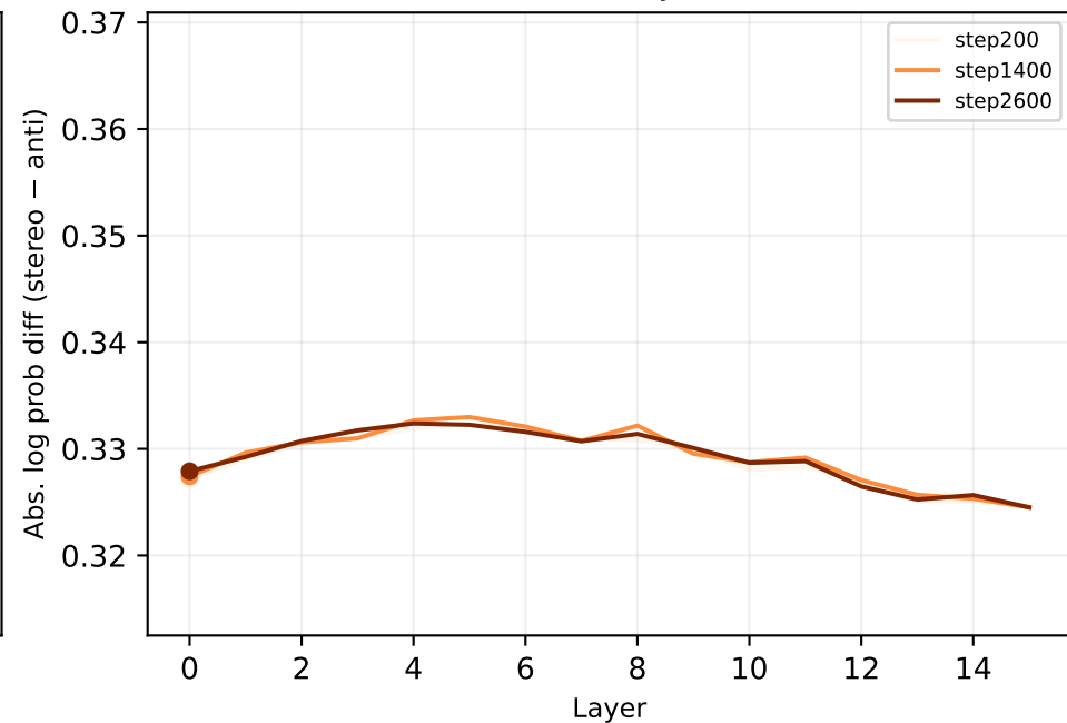
MLP-only
