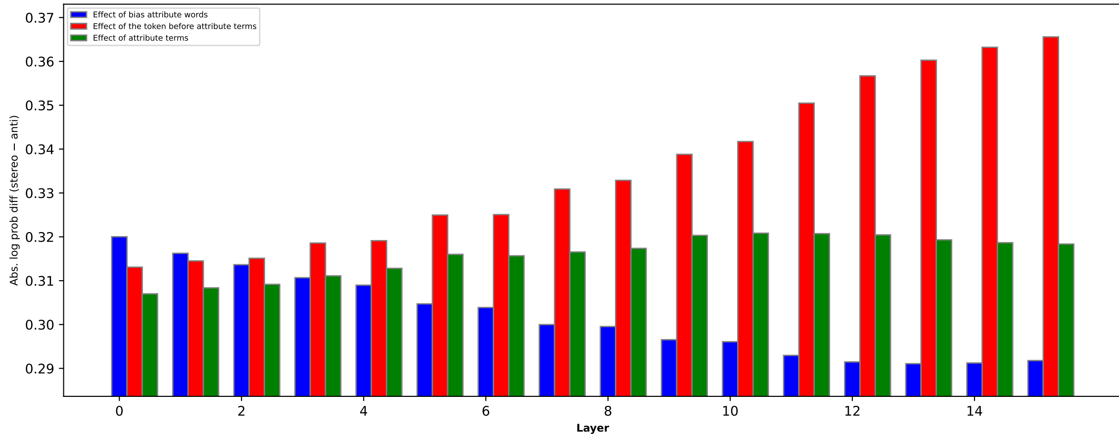
Gender bias effect of different words (OLMo-2-0425-1B [2.4T])
