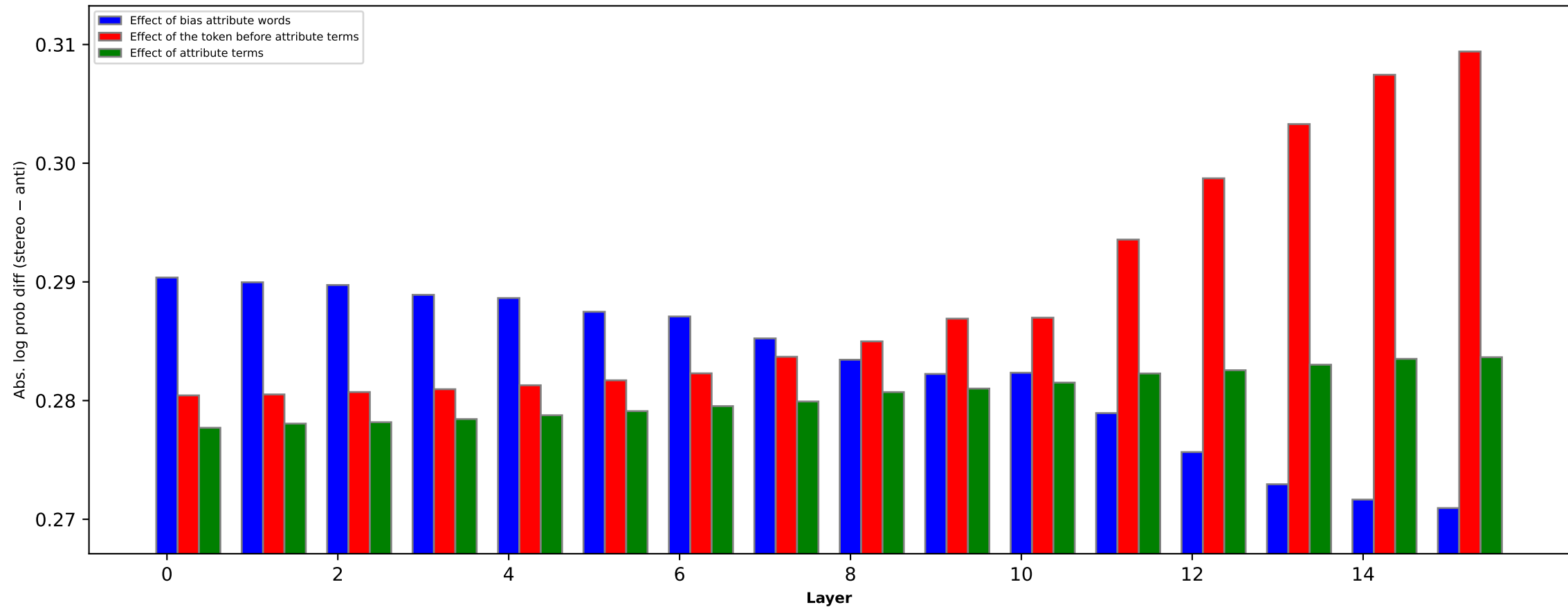
Profession bias effect of different words (OLMo-2-0425-1B [21B])
