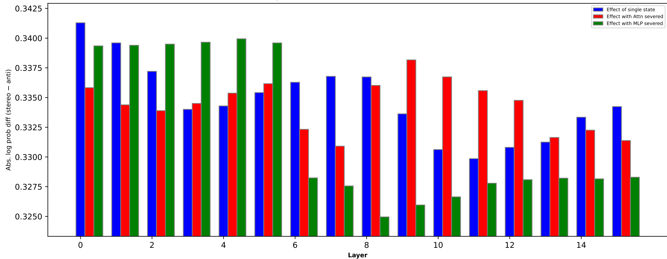
Religion bias effect of states (OLMo-2-0425-1B [21B])
