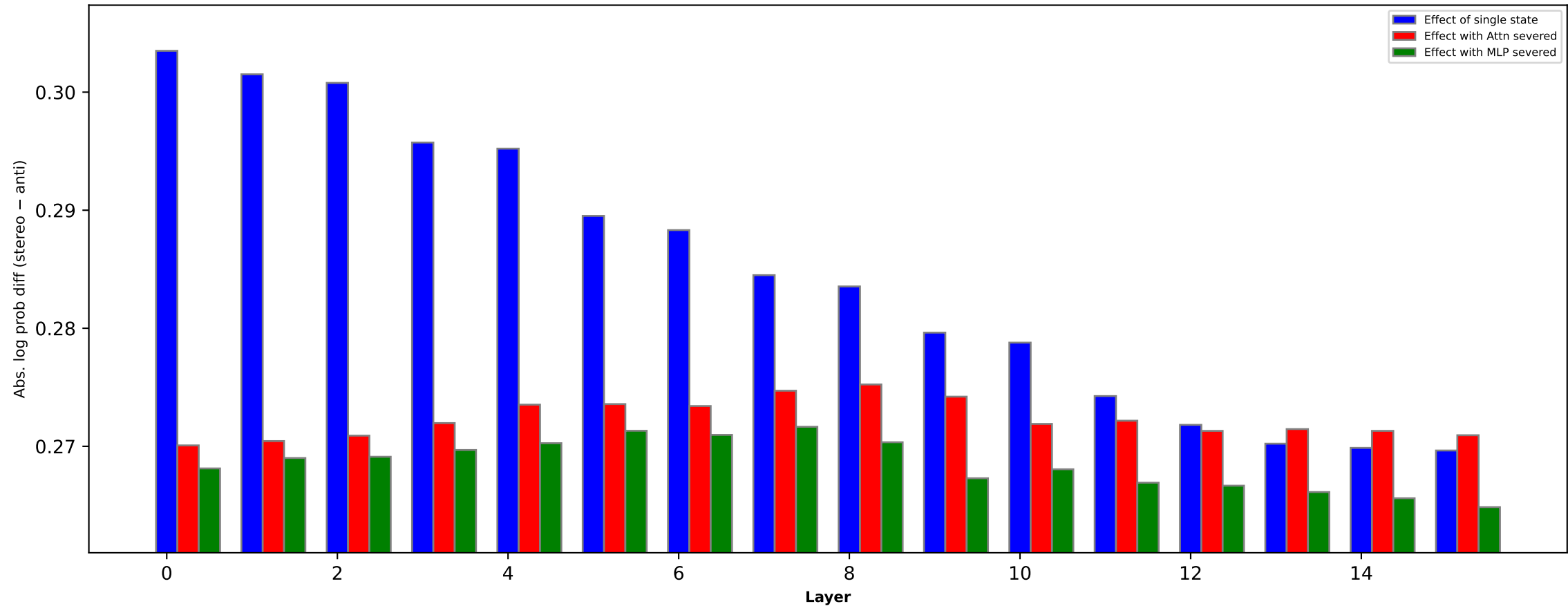
Profession bias effect of states (OLMo-2-0425-1B [4T])
