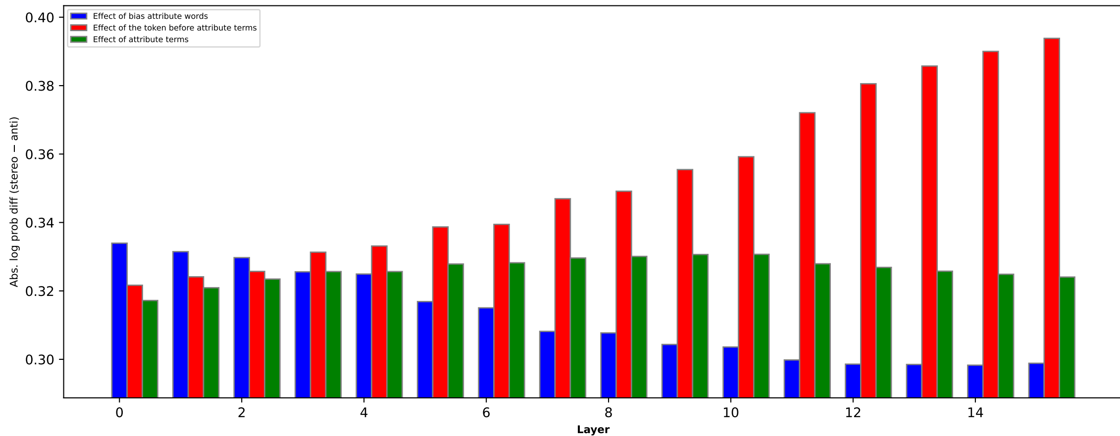
Gender bias effect of different words (OLMo-2-0425-1B [s2-24B])
