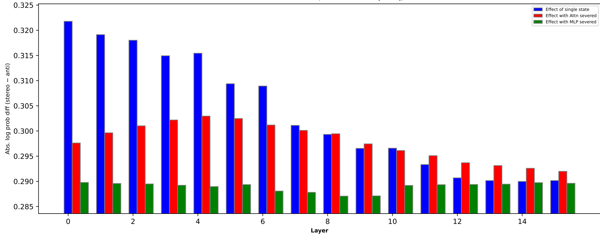
Race bias effect of states (OLMo-2-0425-1B [s2-3B])
