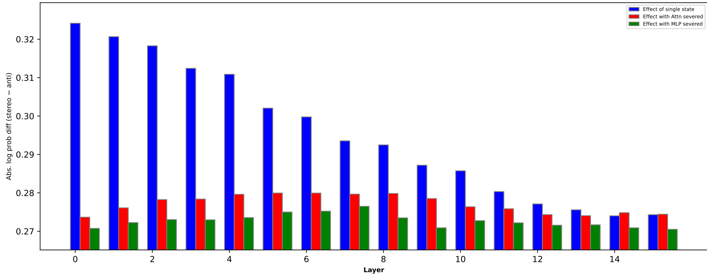
Profession bias effect of states (OLMo-2-0425-1B [s2-51B])
