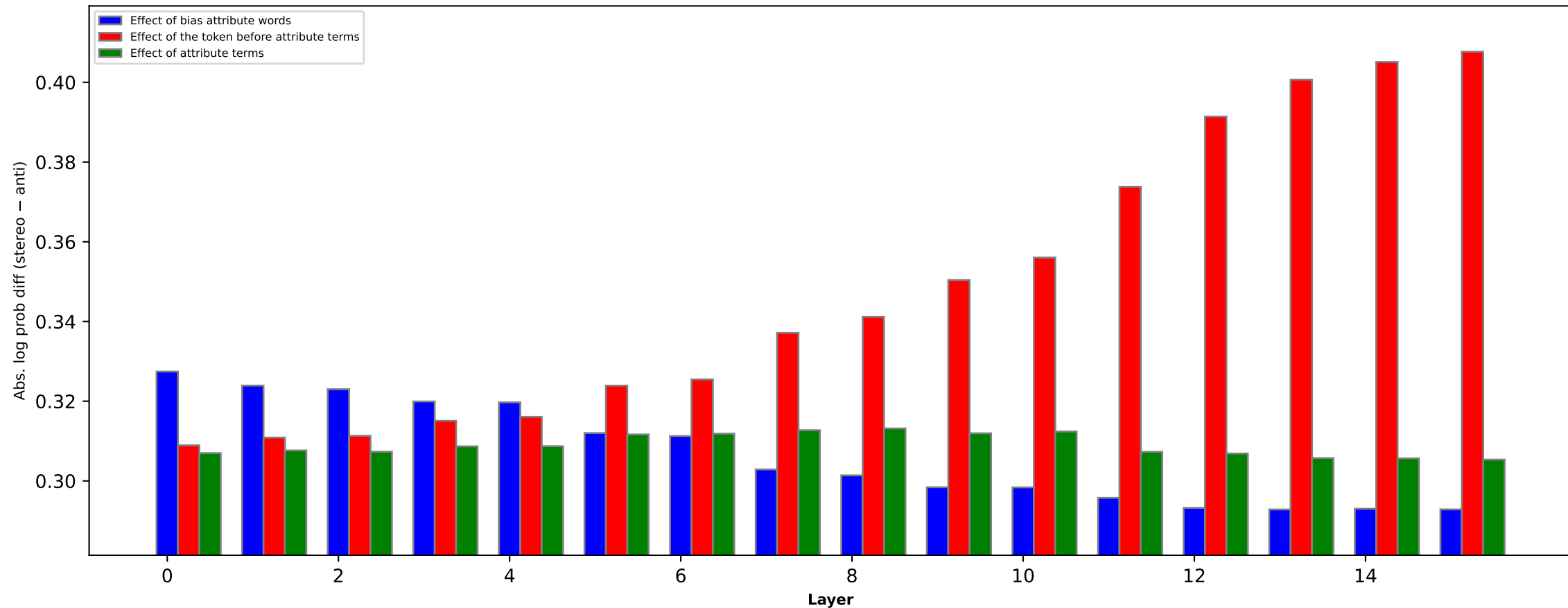
Race bias effect of different words (OLMo-2-0425-1B [s2-51B])
