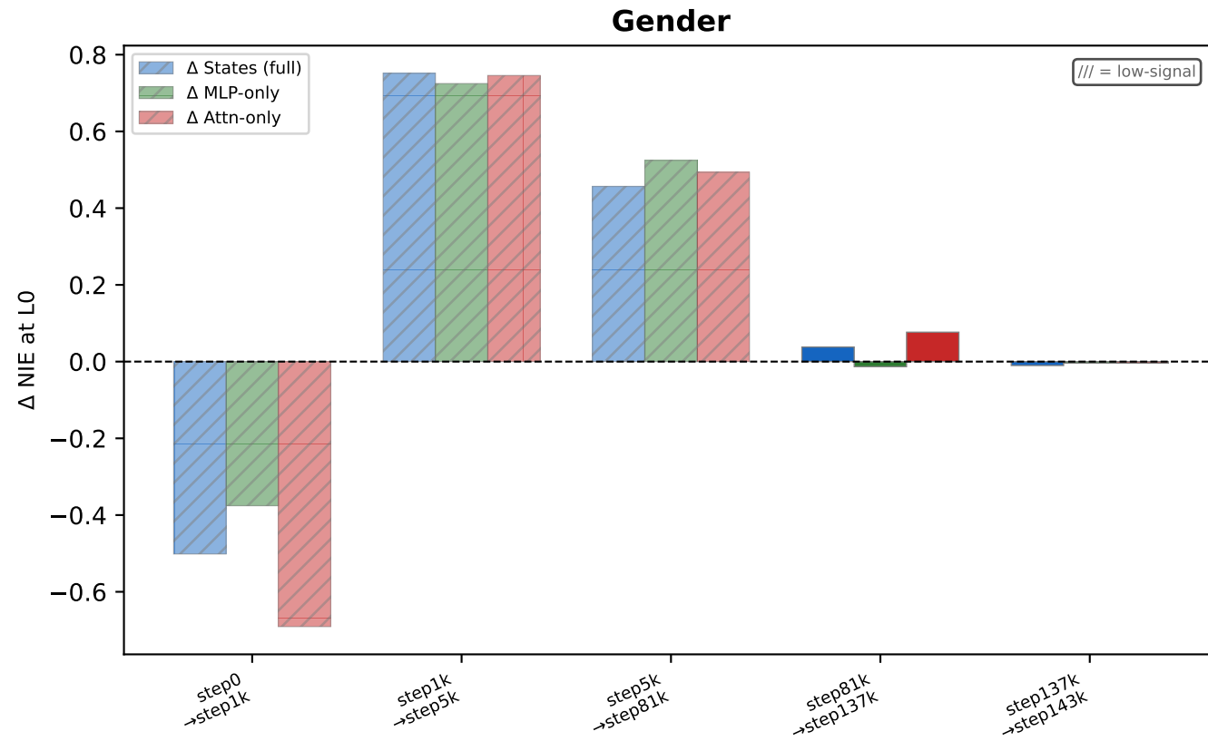
pythia-1b — Change in NIE at L0 per Training Interval Each group: \Delta NIE-L0 for States / MLP-only / Attn-only (positive = more causal effect gained, negative = lost)
