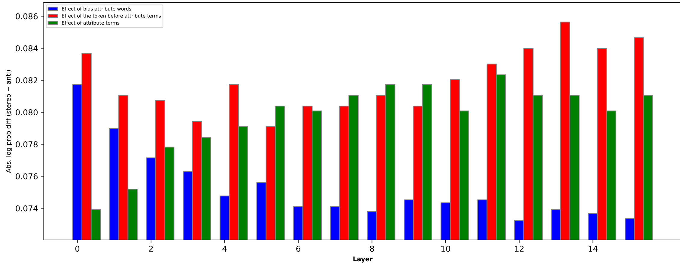
Religion bias effect of different words (pythia-1b [step0])
