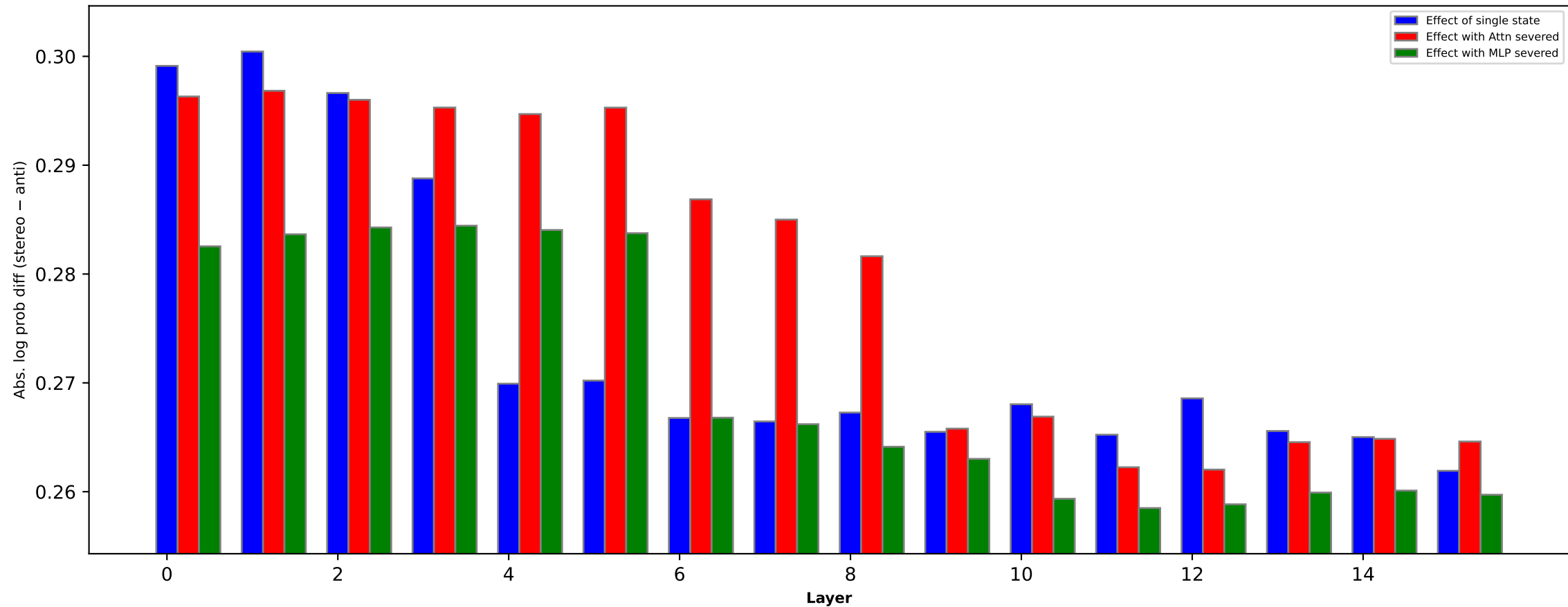
Race bias effect of states (pythia-1b [step137k])
