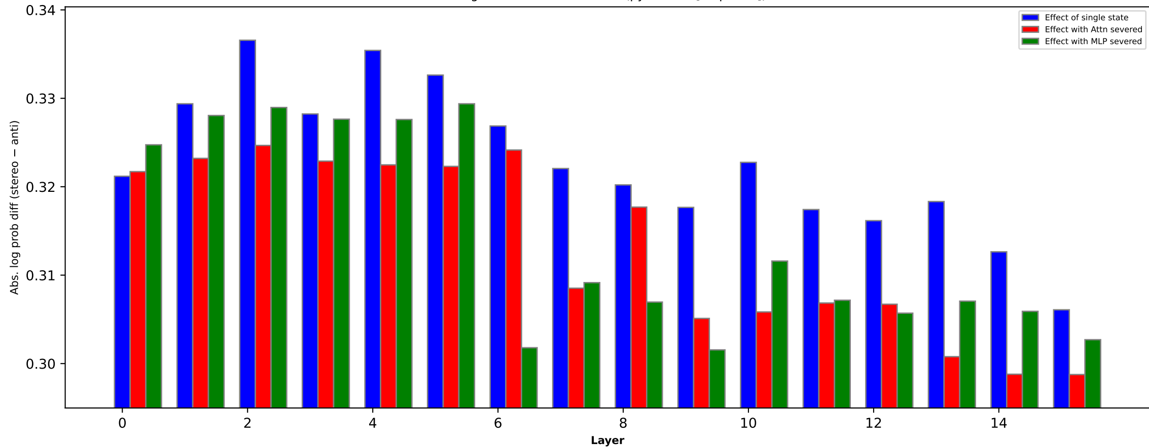
Religion bias effect of states (pythia-1b [step137k])
