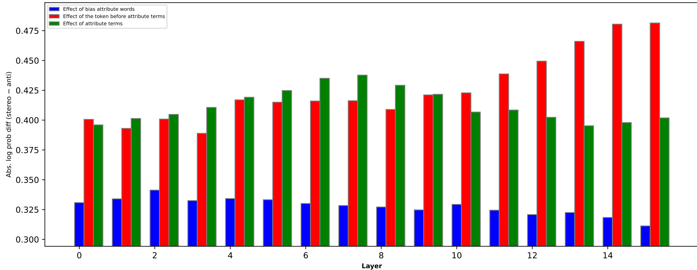
Religion bias effect of different words (pythia-1b [step143k])
