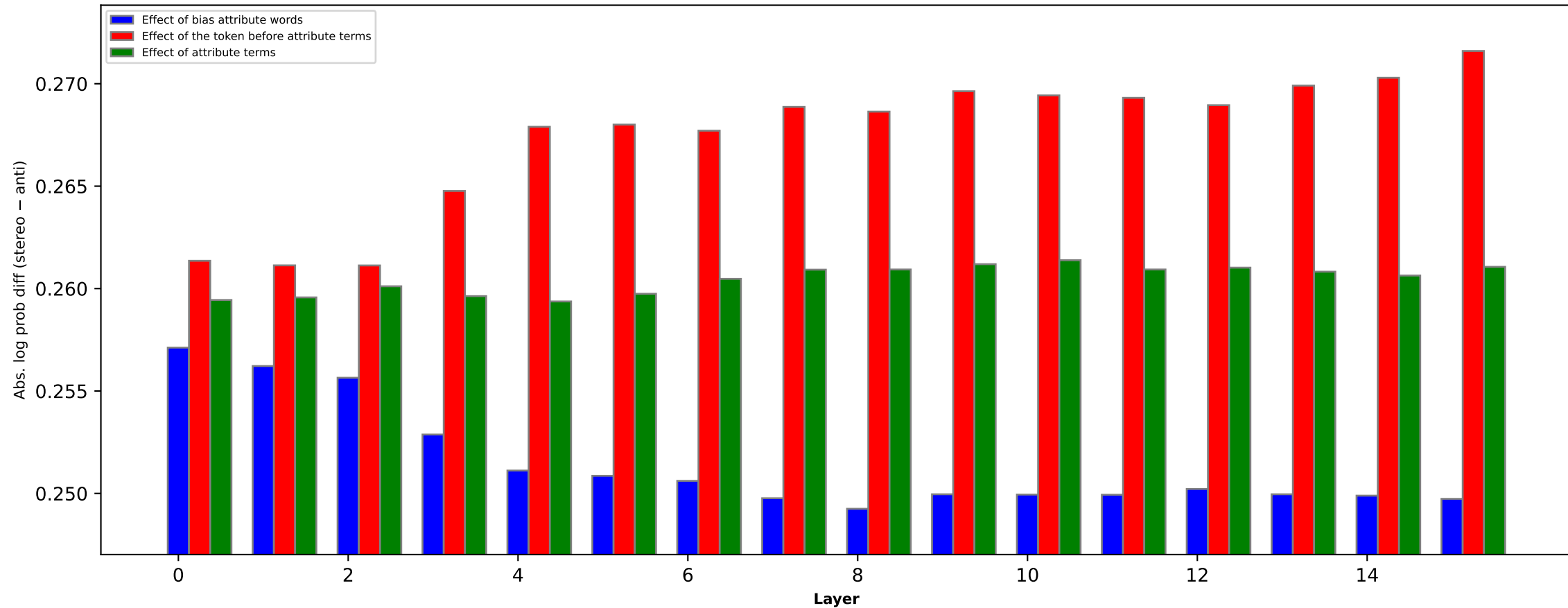
Profession bias effect of different words (pythia-1b [step1k])
