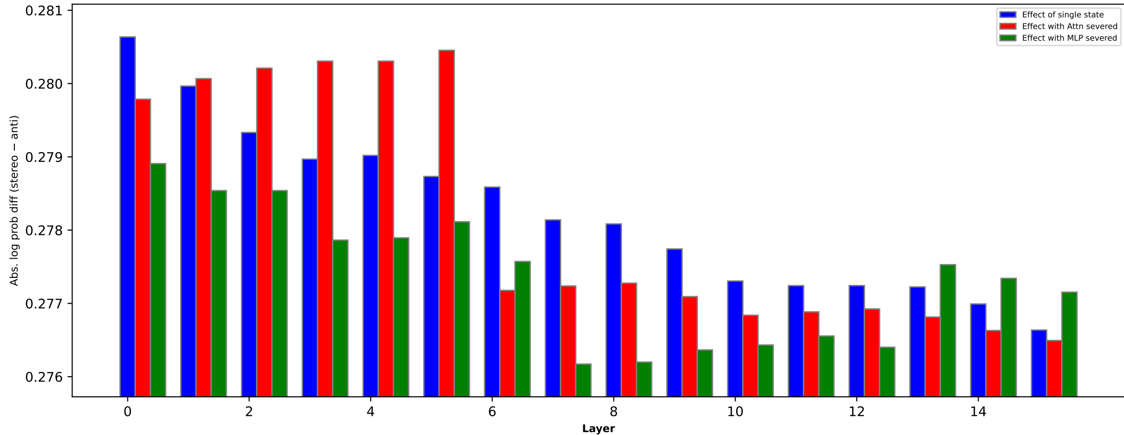
Race bias effect of states (pythia-1b [step1k])
