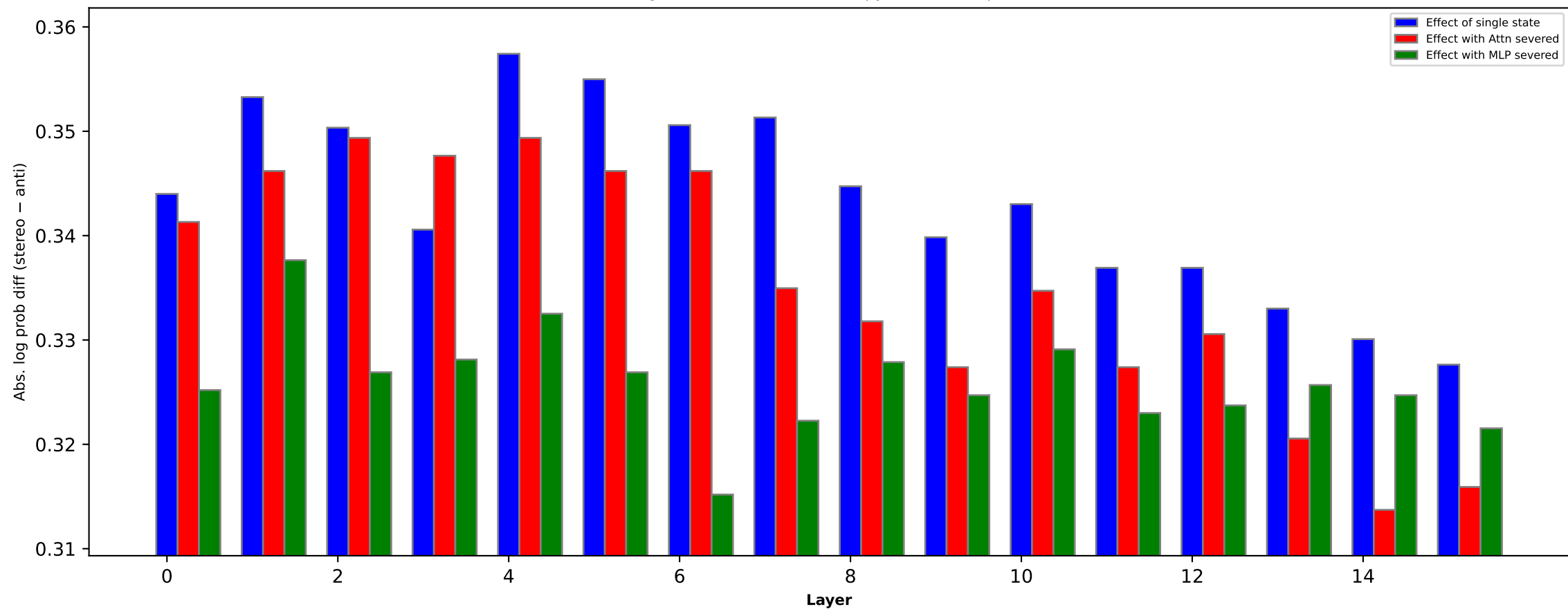
Religion bias effect of states (pythia-1b [step81k])
