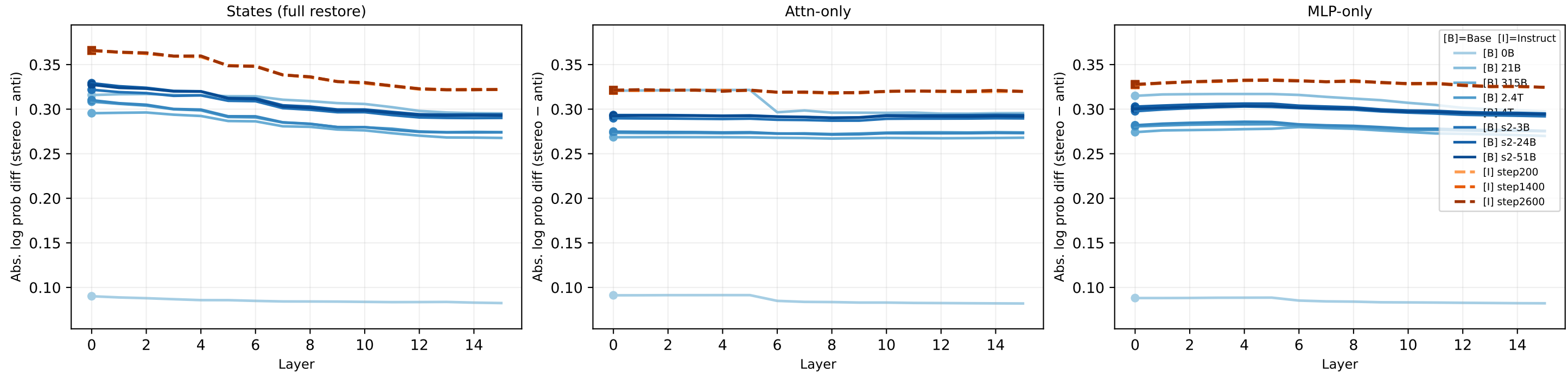
OLMo-2-0425-1B — Race bias: Base (solid) vs Instruct (dashed) Each line = one checkpoint. X = layer, Y = abs. log prob diff (stereo – anti). Y-axis shared.
