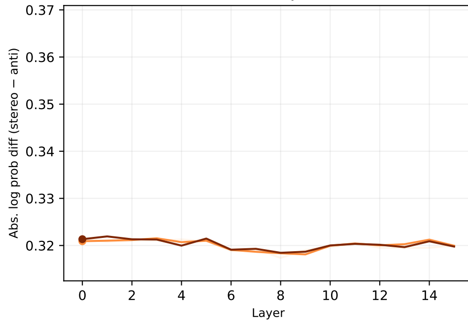
Attn-only
