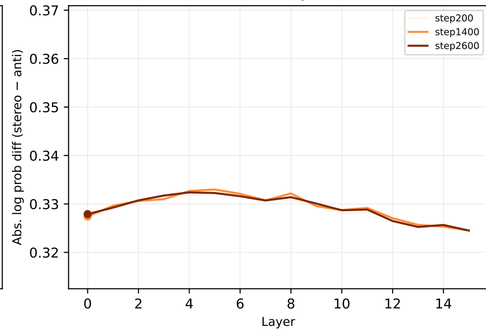
MLP-only
