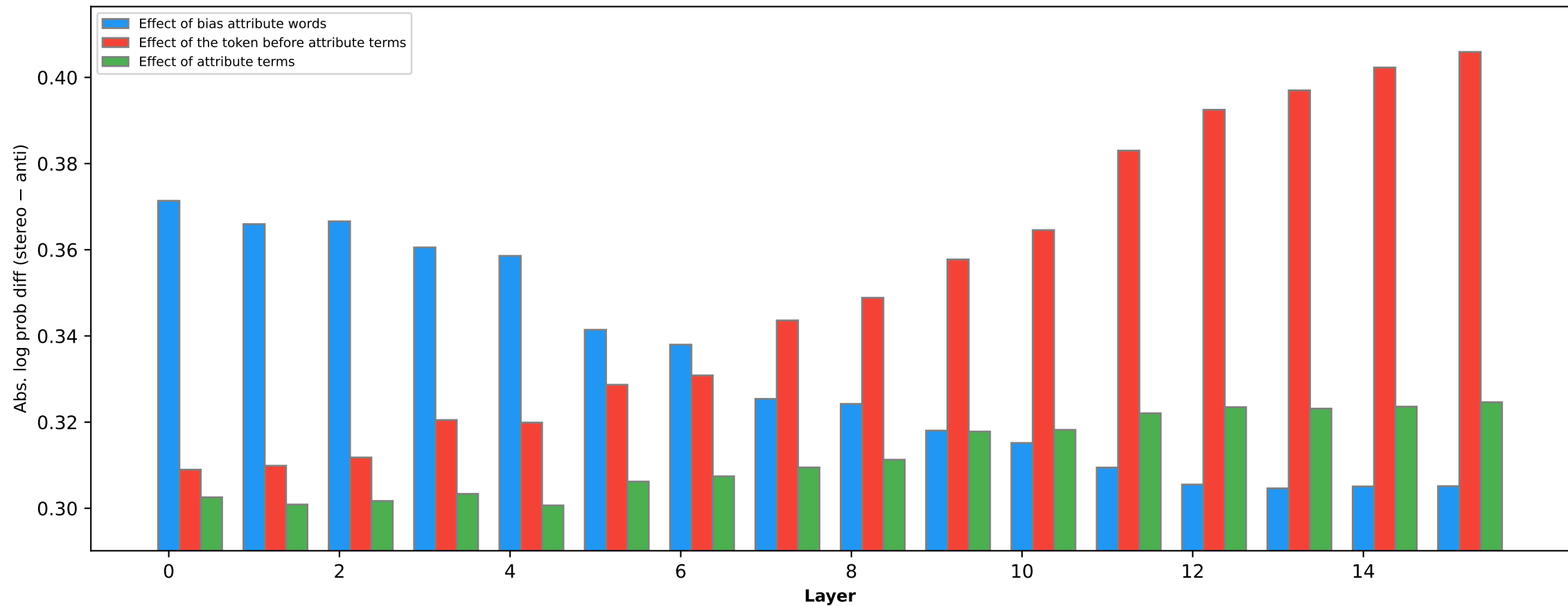
Profession bias effect of different words (OLMo-2-0425-1B-Instruct [step1400])
