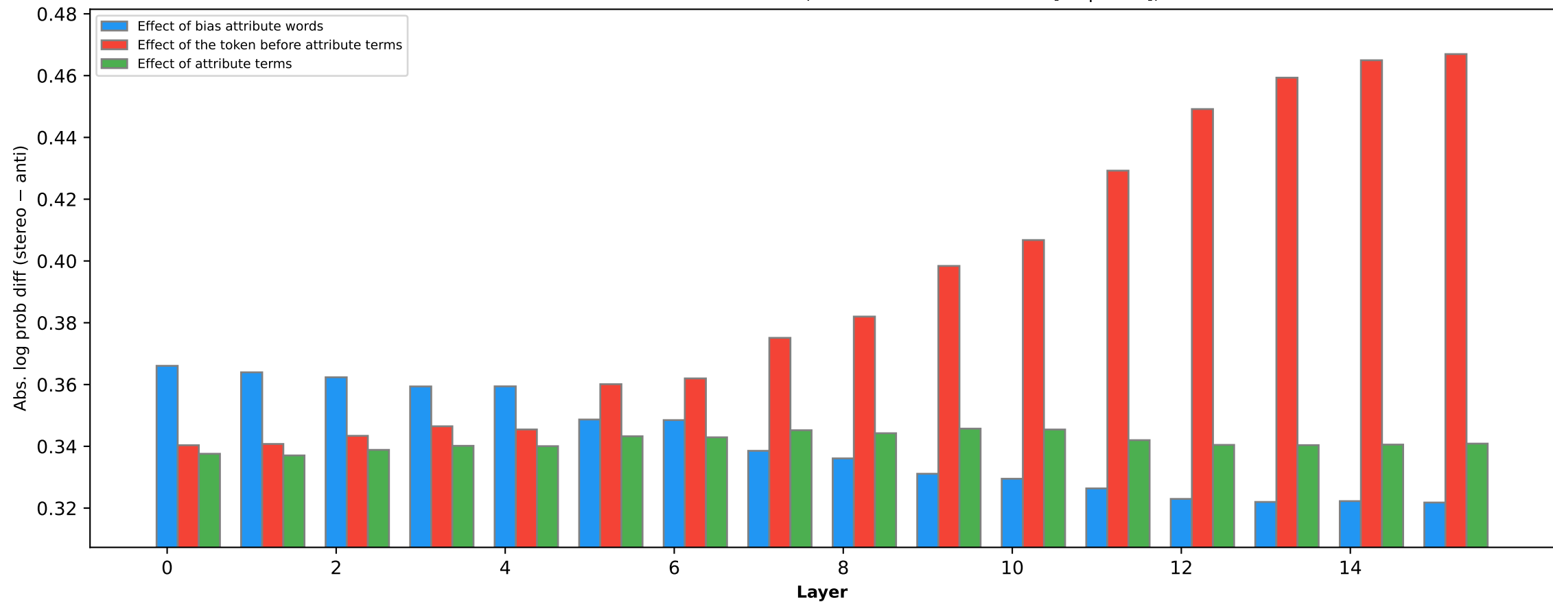
Race bias effect of different words (OLMo-2-0425-1B-Instruct [step1400])
