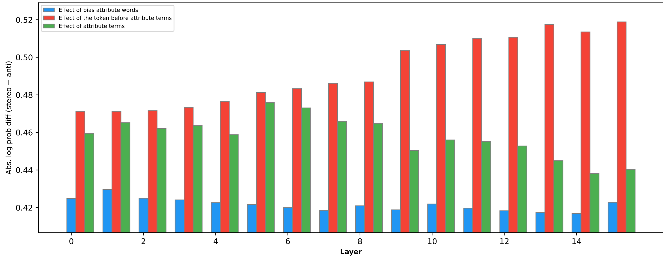
Religion bias effect of different words (OLMo-2-0425-1B-Instruct [step200])
