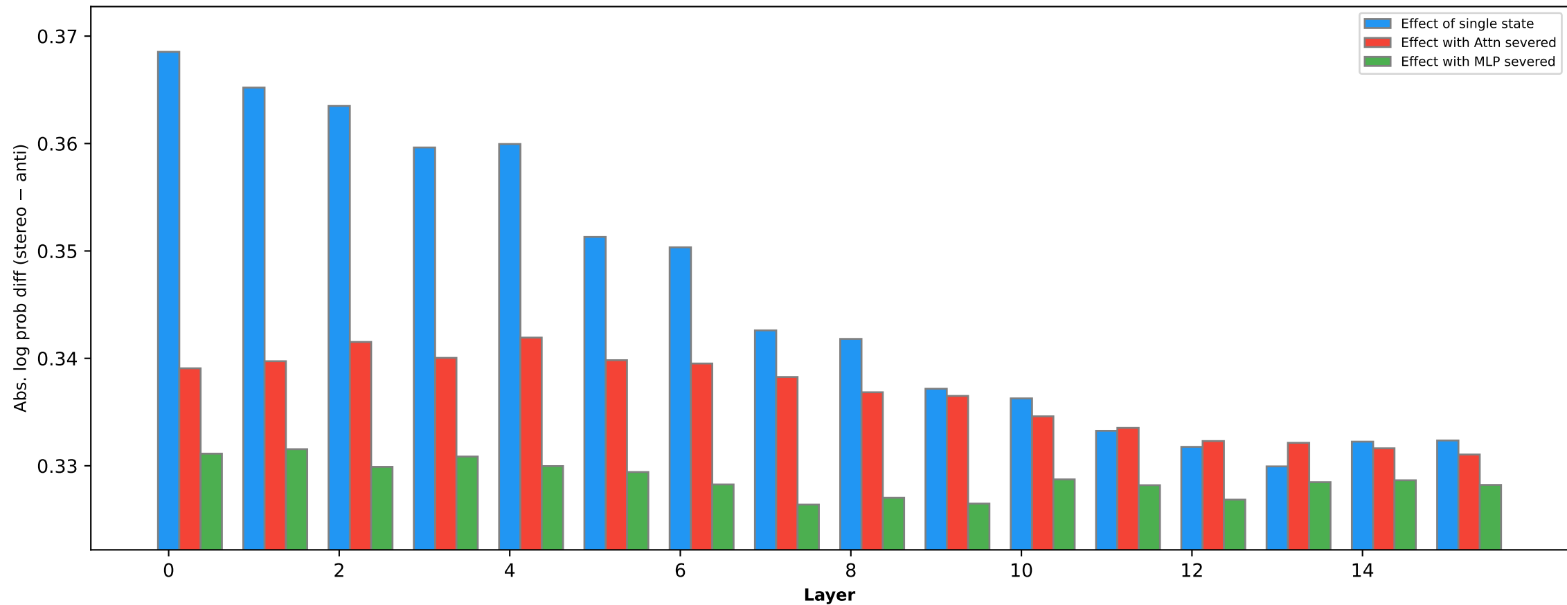
Gender bias effect of states (OLMo-2-0425-1B-Instruct [step2600])
