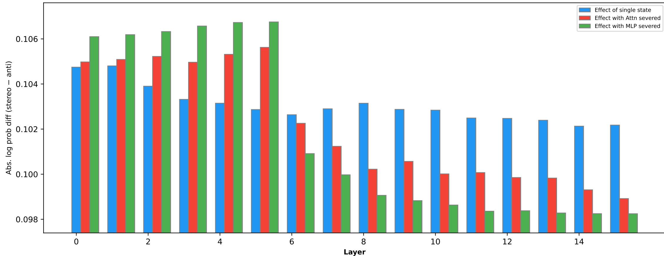
Gender bias effect of states (OLMo-2-0425-1B [0B])
