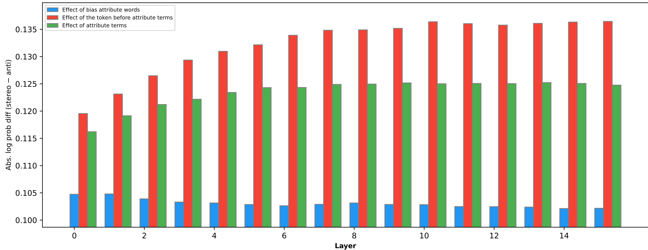
Gender bias effect of different words (OLMo-2-0425-1B [0B])
