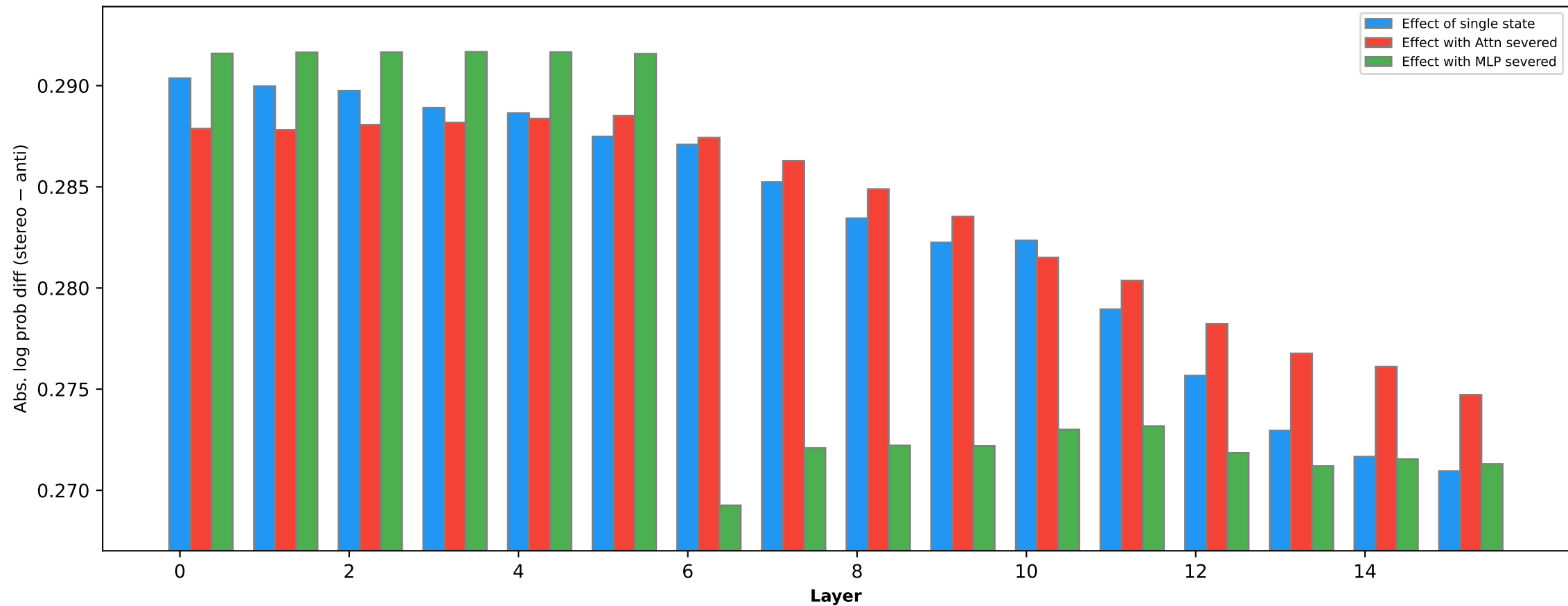
Profession bias effect of states (OLMo-2-0425-1B [21B])
