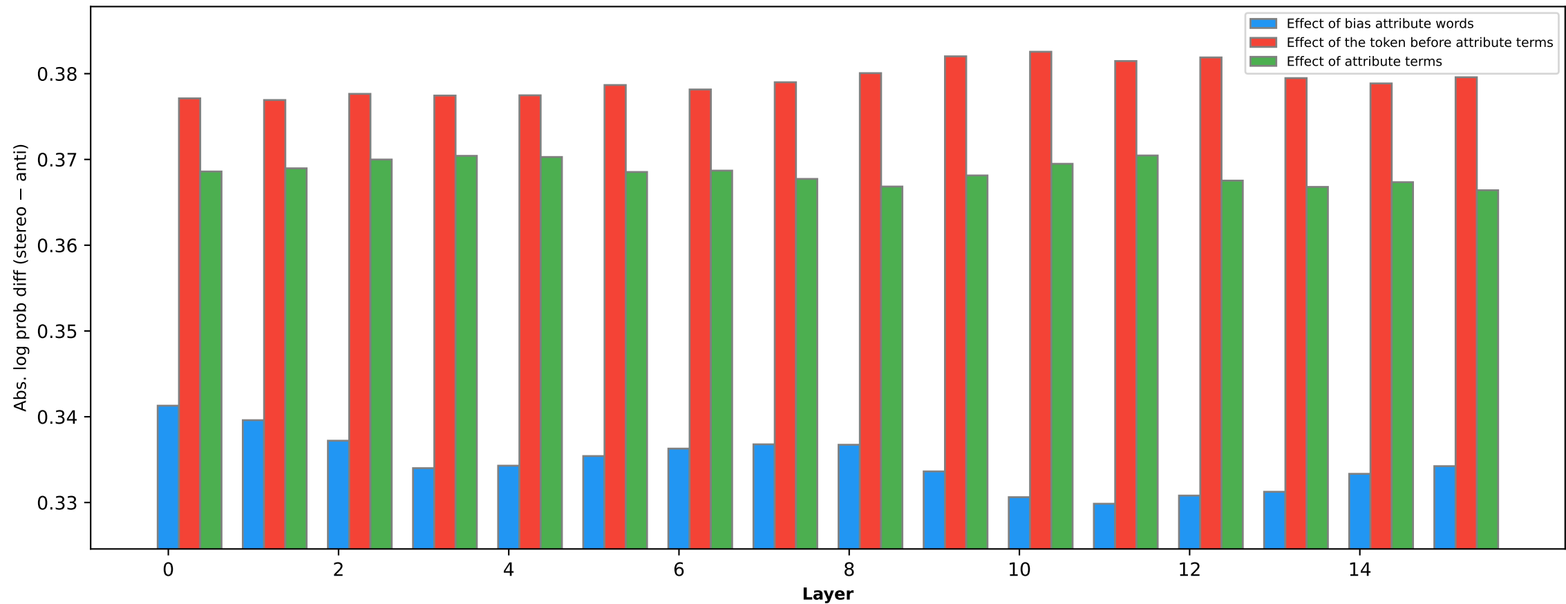
Religion bias effect of different words (OLMo-2-0425-1B [21B])
