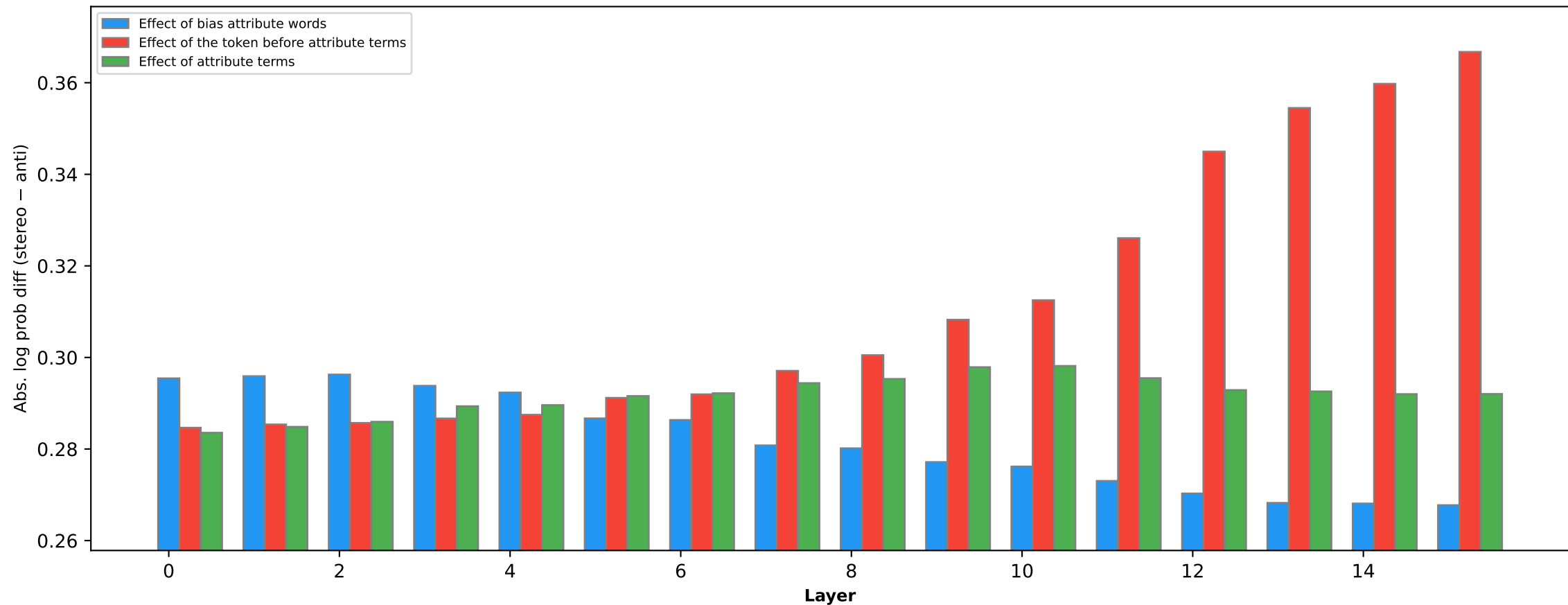
Race bias effect of different words (OLMo-2-0425-1B [315B])
