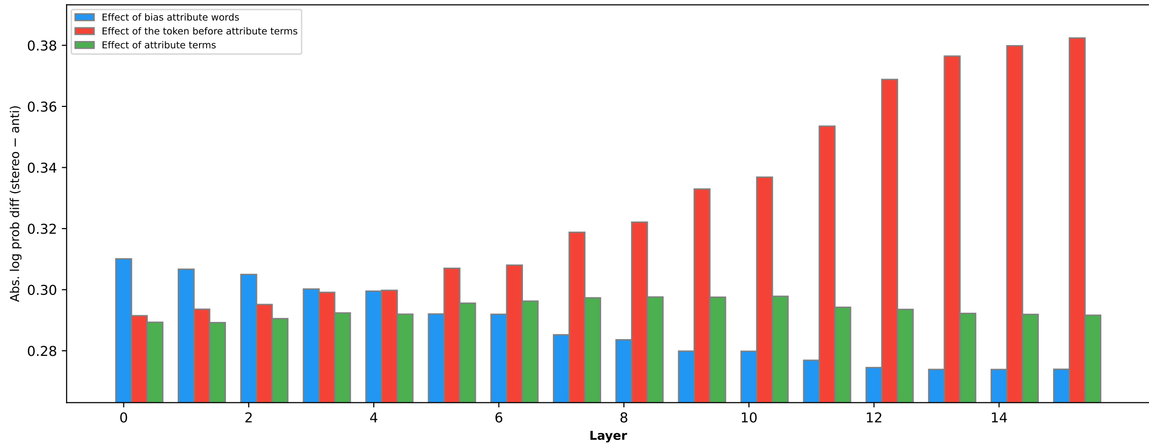
Race bias effect of different words (OLMo-2-0425-1B [4T])
