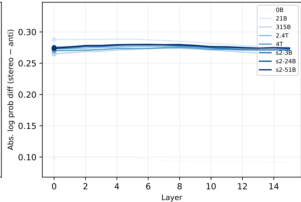
MLP-only
