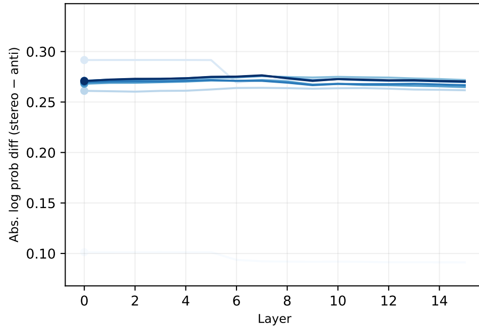
Attn-only
