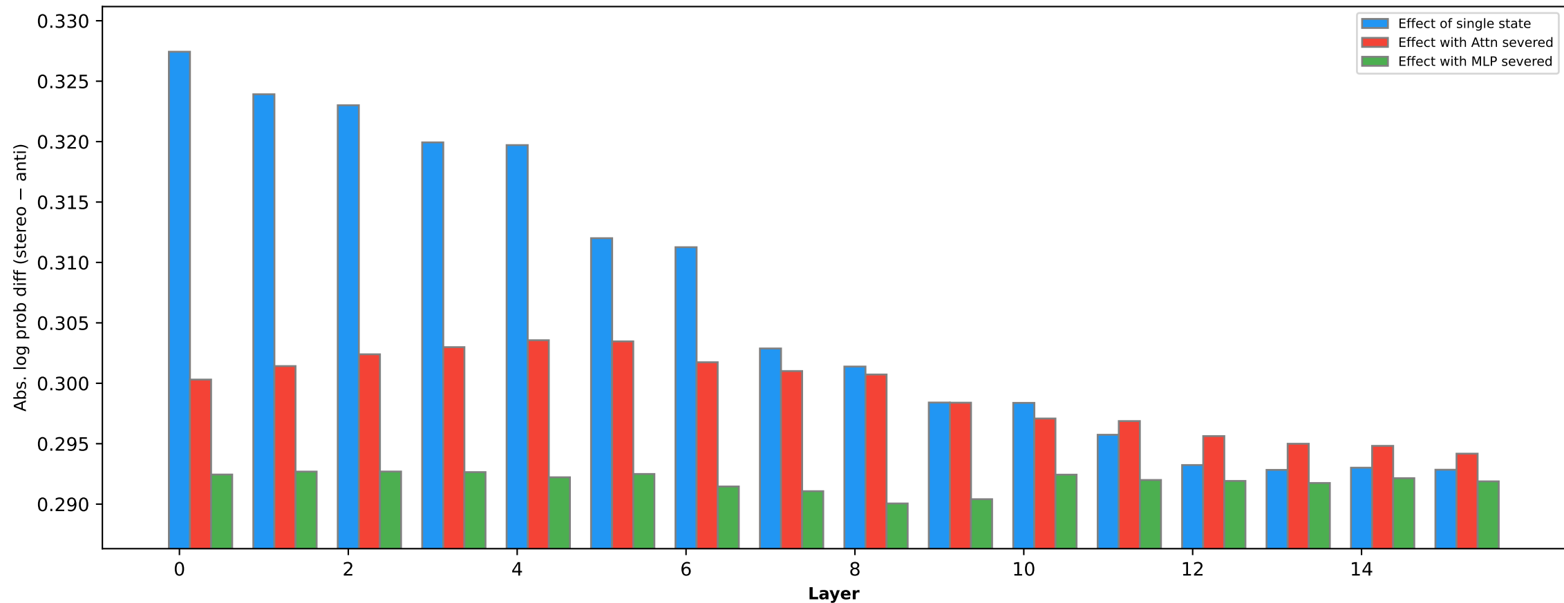
Race bias effect of states (OLMo-2-0425-1B [s2-51B])
