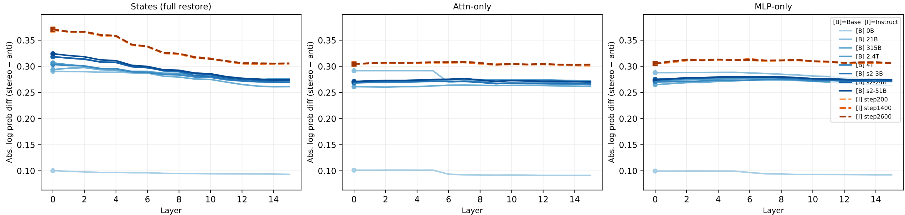
OLMo-2-0425-1B — Profession bias: Base (solid) vs Instruct (dashed) Each line = one checkpoint. X = layer, Y = abs. log prob diff (stereo – anti). Y-axis shared.
