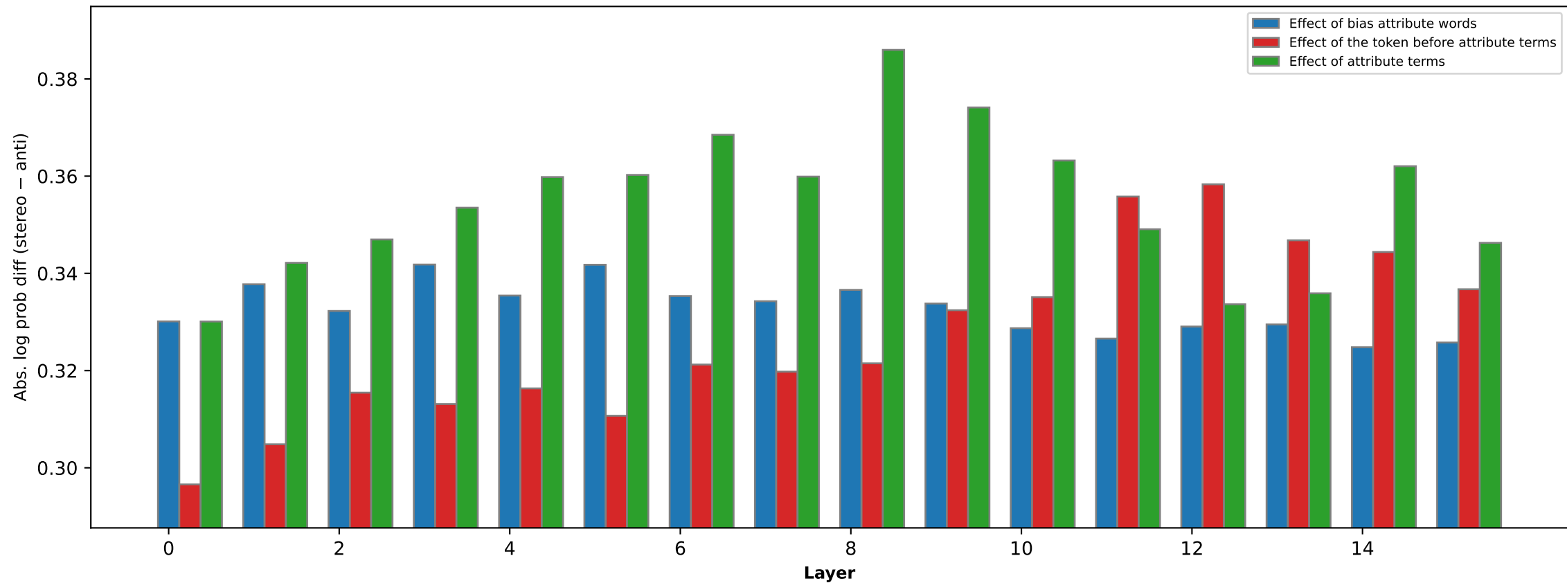
Gender — Pre → Post Base activations patched into instruct model
