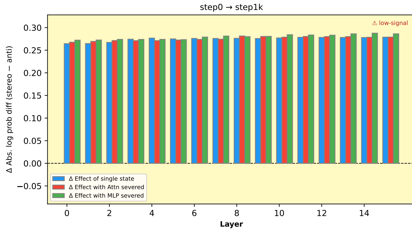
pythia-1b — Religion bias: \Delta per layer vs. previous checkpoint Bars show change in abs. log prob diff (curr – prev) at each layer. Positive = more causal effect acquired. Y-axis fixed across all intervals.
