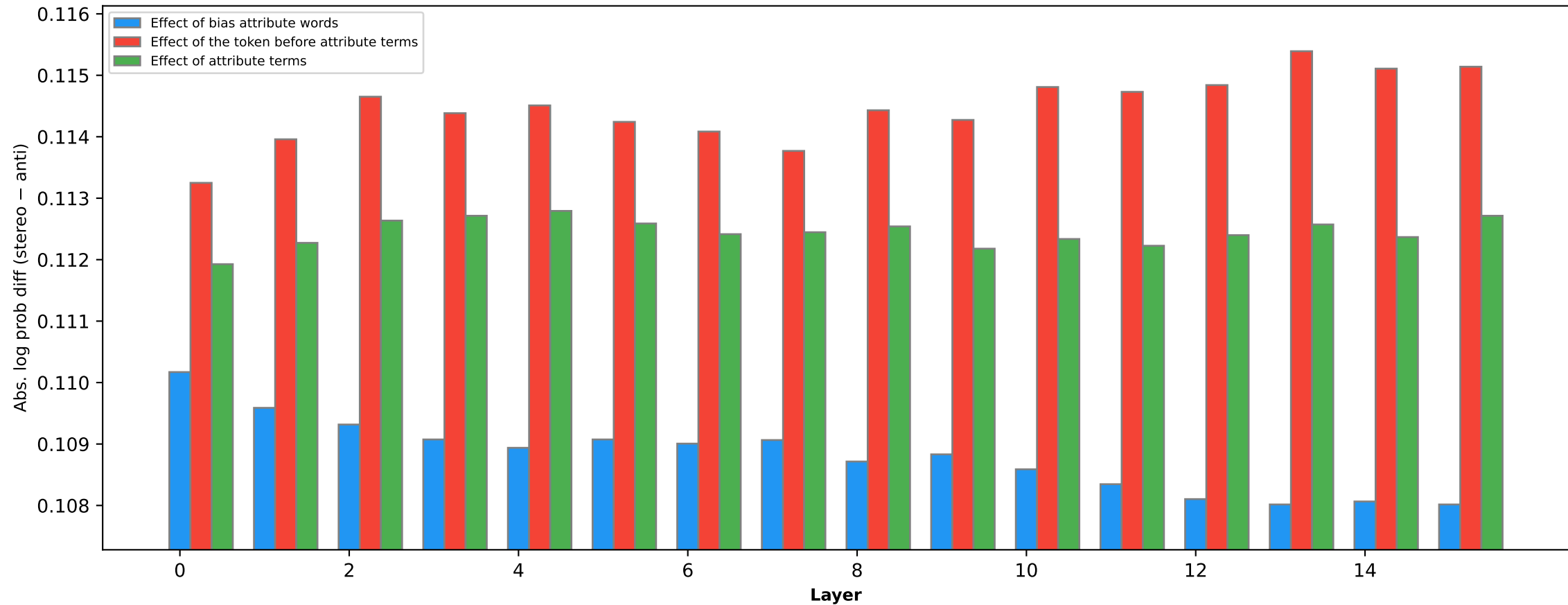
Profession bias effect of different words (pythia-1b [step0])
