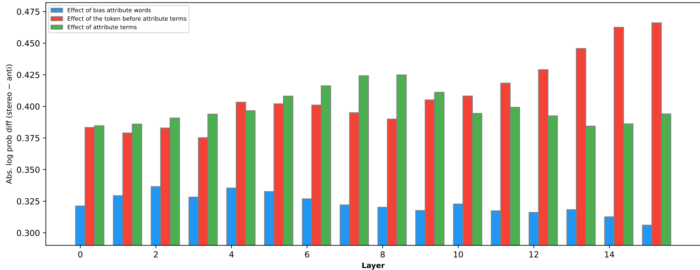
Religion bias effect of different words (pythia-1b [step137k])
