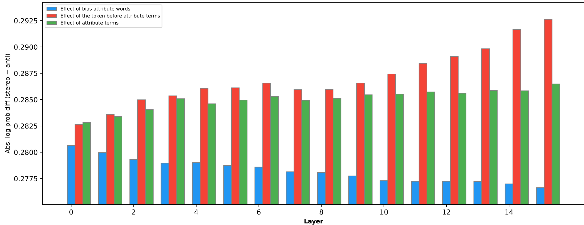
Race bias effect of different words (pythia-1b [step1k])
