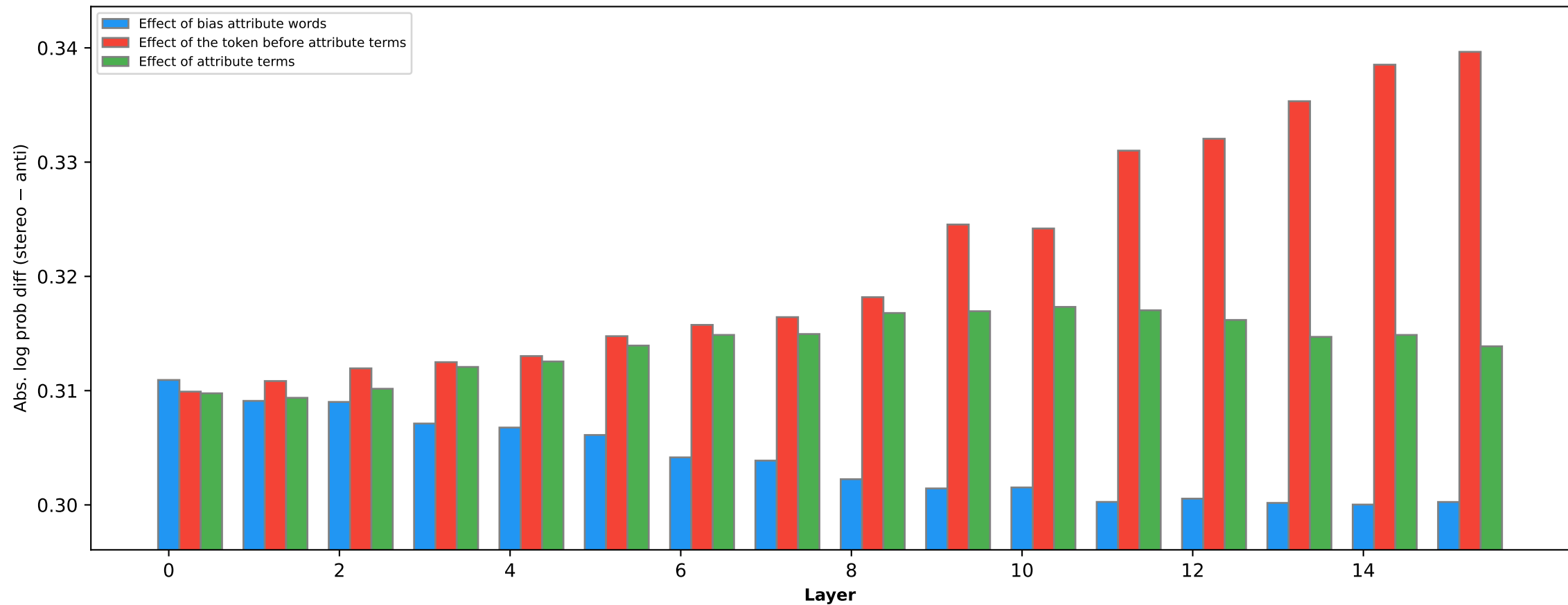
Race bias effect of different words (pythia-1b [step5k])
