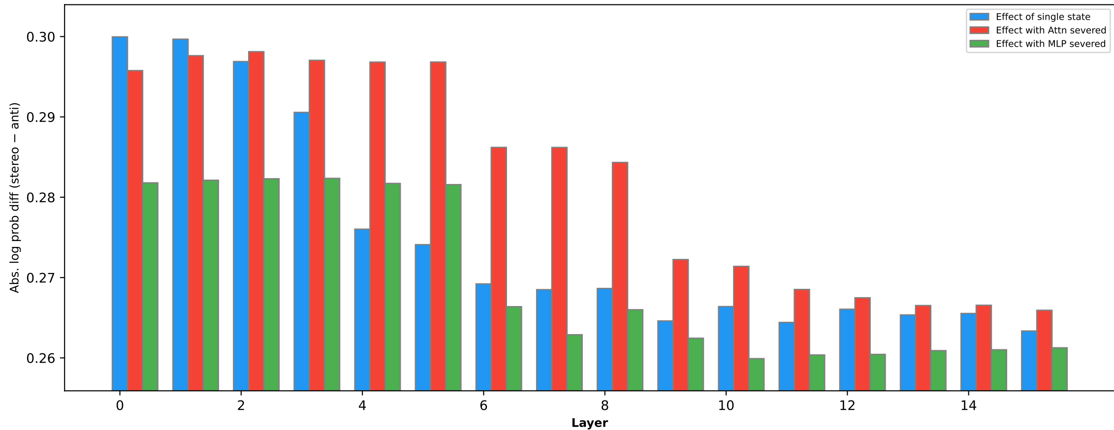
Race bias effect of states (pythia-1b [step81k])
