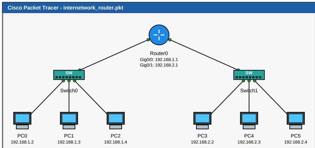
Packet Tracer view of Part (a)
