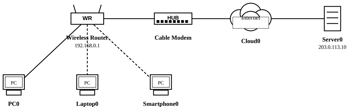
Fig 2: Wireless router with DHCP and internet cloud (Part b) - dotted lines are wireless links
