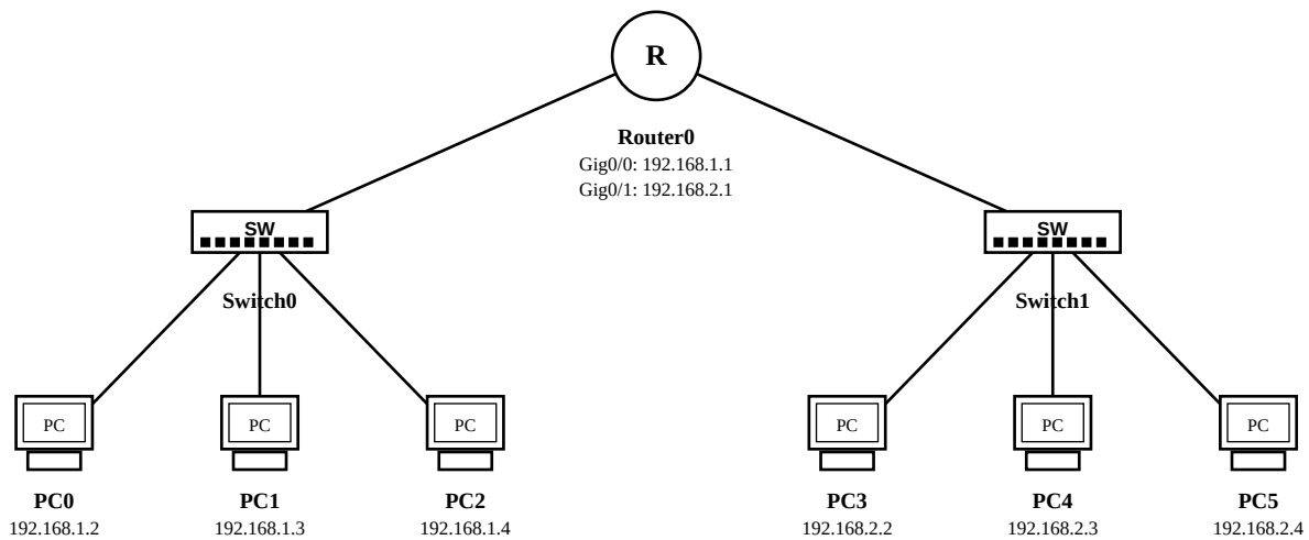
Fig 1: Internetwork of two LANs connected by a router (Part a)
