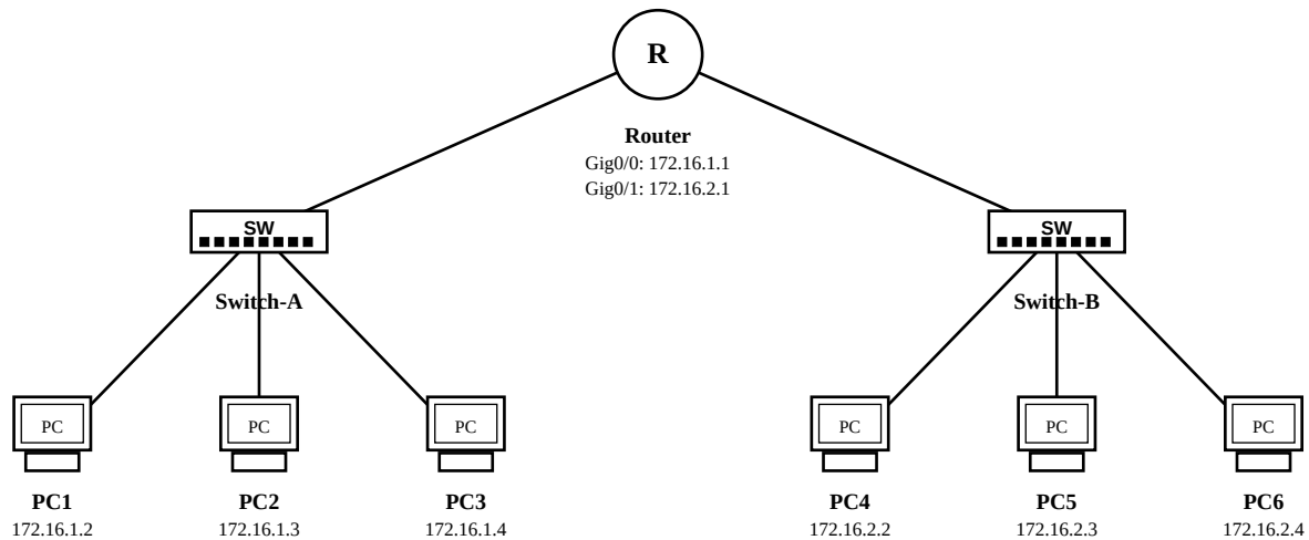
Fig 3: Lab inter-network using switches, router and Ethernet cables (Part c)
