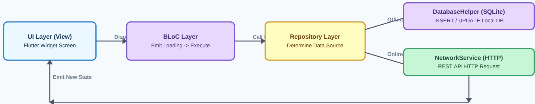
Flow 3.1: BLoC State Management Architecture Flow (Clean Architecture)
