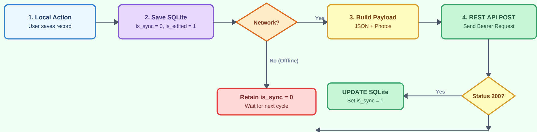
Flow 3.2: Offline-First Synchronization State Machine Logic
