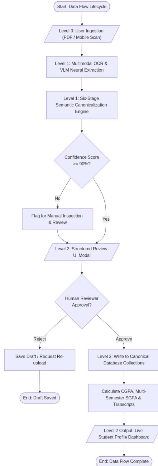
Fig. 2. Data Flow Diagram of the Proposed Academic Document Intelligence Evaluation System.
