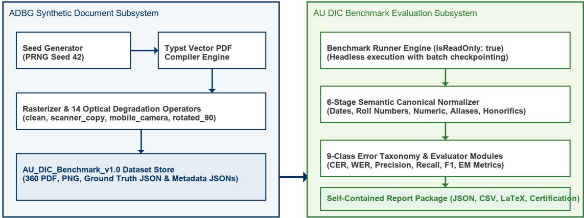
Fig. 1. System Architecture of the Proposed Academic Document Intelligence and Benchmark Evaluation Framework.
