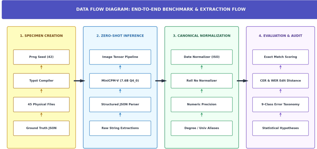
Fig. 2. Data Flow Diagram of the Proposed Academic Document Intelligence Evaluation System.
