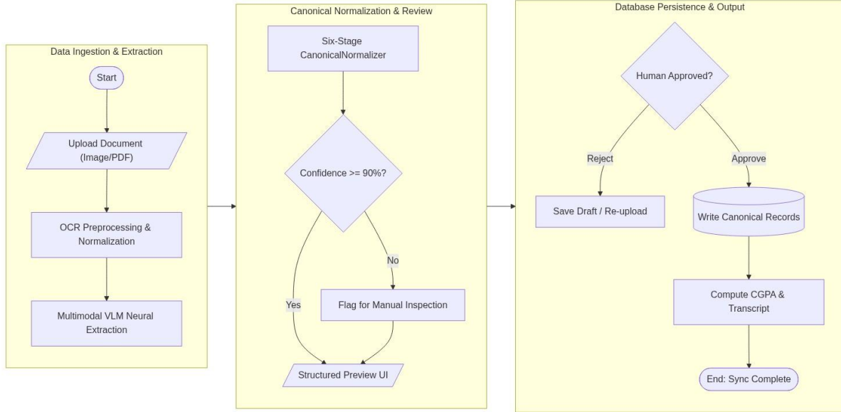
Fig. 2. Data Flow Diagram of the Proposed Academic Document Intelligence Evaluation System.
