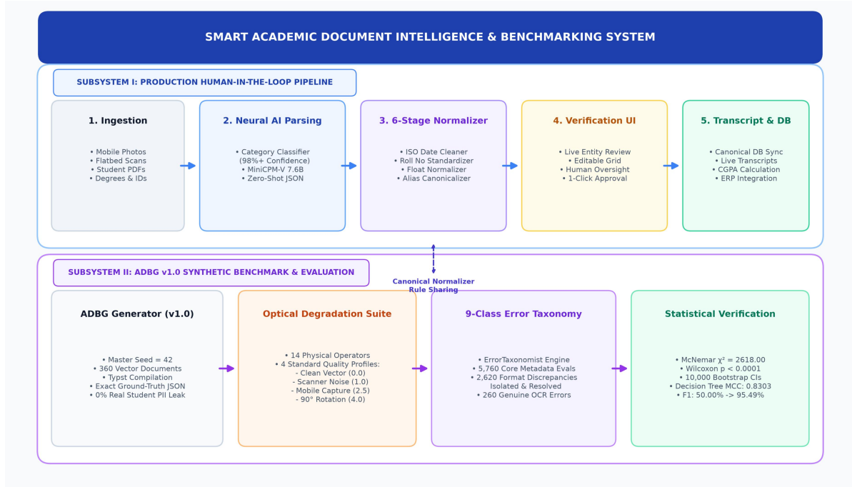
Fig. 1. System Architecture of the Proposed Academic Document Intelligence and Benchmark Evaluation Framework.
