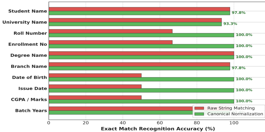
Fig. 7. Field-by-Field Accuracy Improvement Comparing Raw String Matching Against Canonical Normalization.
