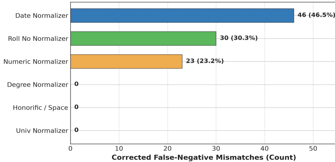
Fig. 6. Total False-Negative Field Mismatches Resolved by Each Individual Domain Normalizer Rule.
