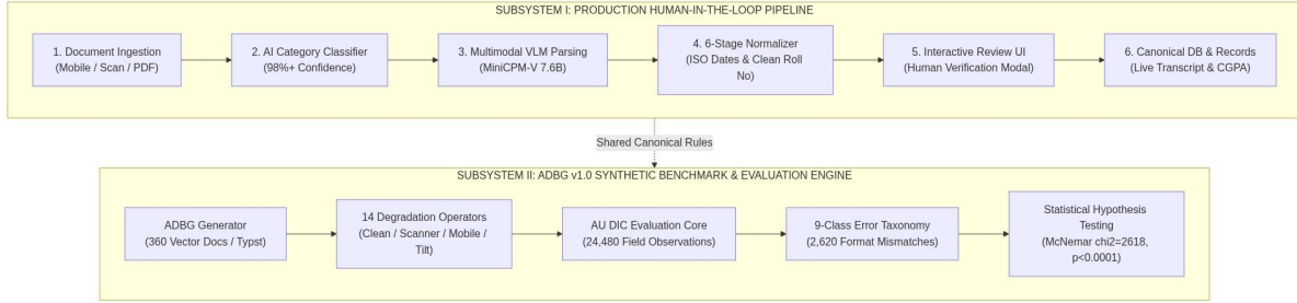
Fig. 1. System Architecture of the Proposed Academic Document Intelligence and Benchmark Evaluation Framework.
